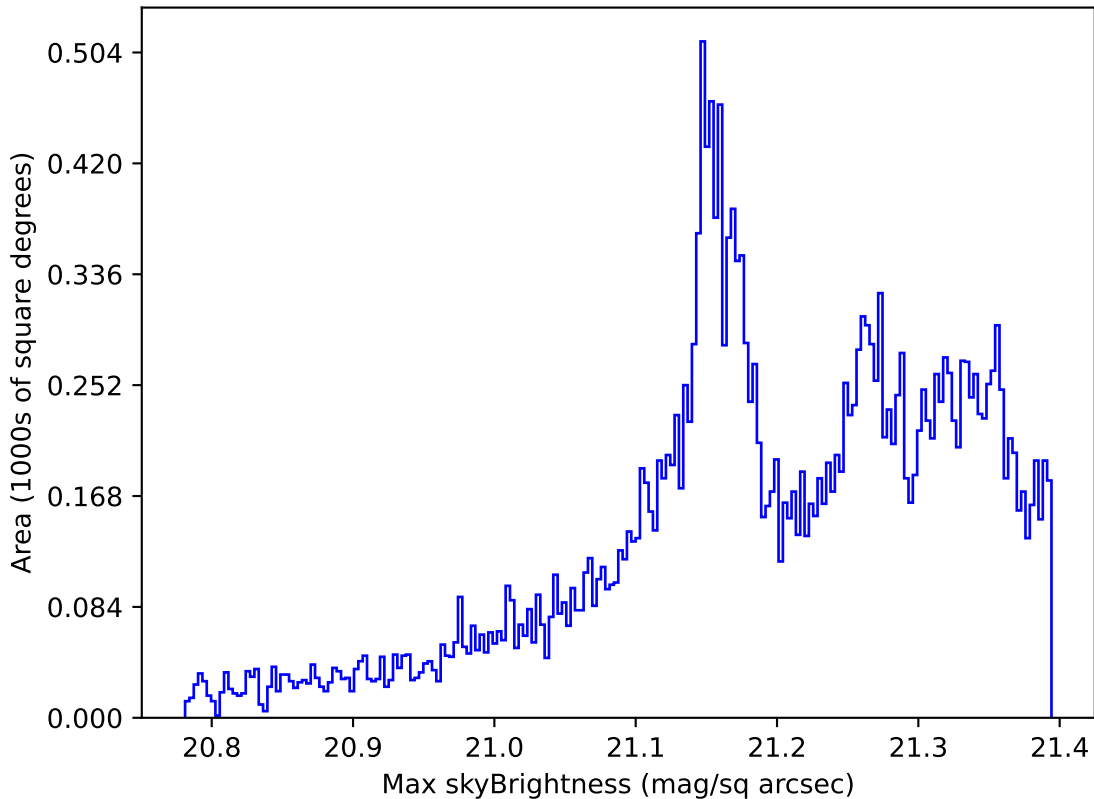
baseline_v3.2_10yrs All sky r band: Max skyBrightness
