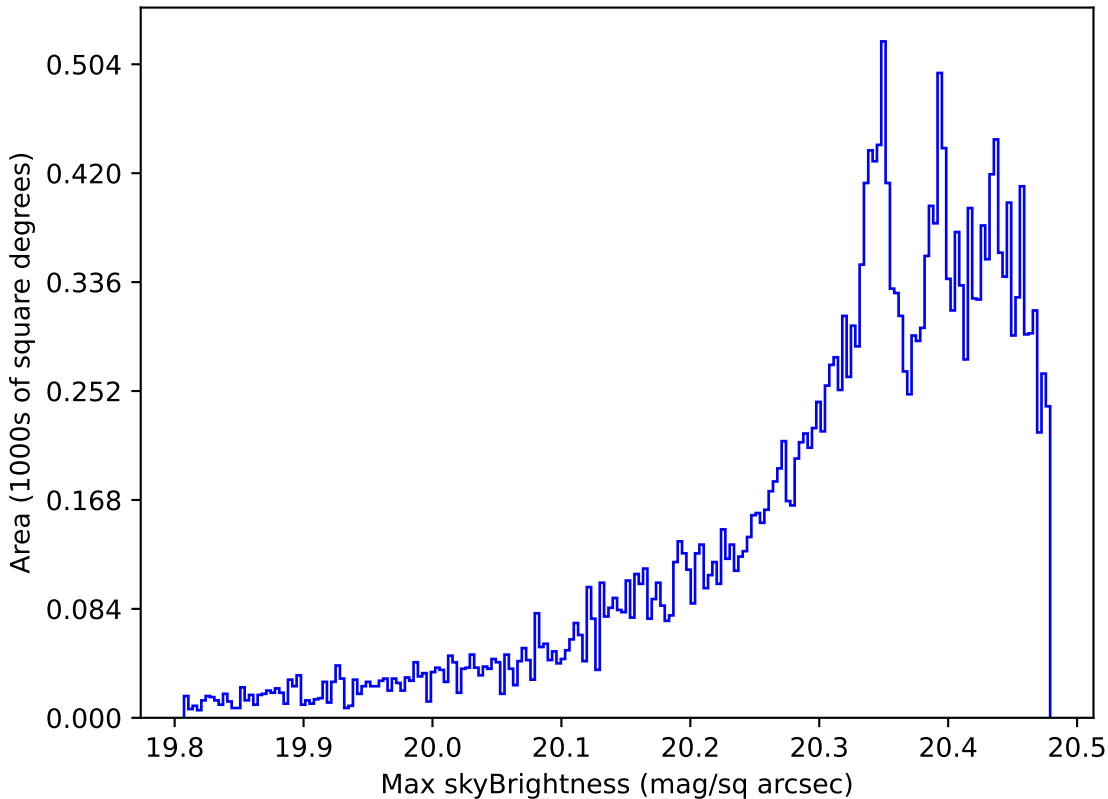
baseline_v3.2_10yrs All sky i band: Max skyBrightness
