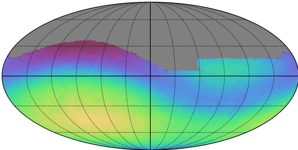
baseline_v3.2_10yrs All sky g band: Max skyBrightness
