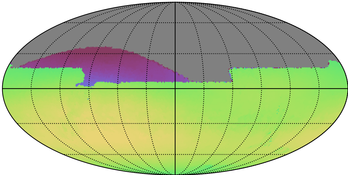
baseline_v3.2_10yrs All sky all bands: Max skyBrightness
