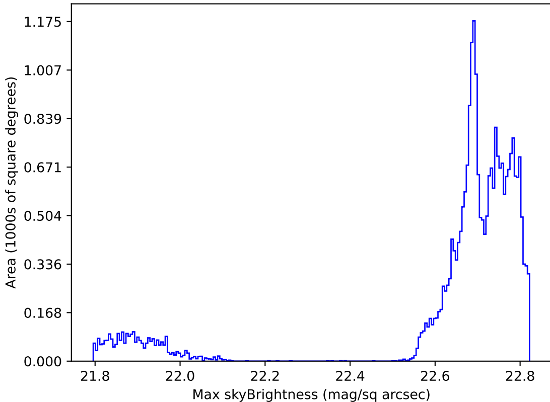
baseline_v3.2_10yrs All sky all bands: Max skyBrightness
