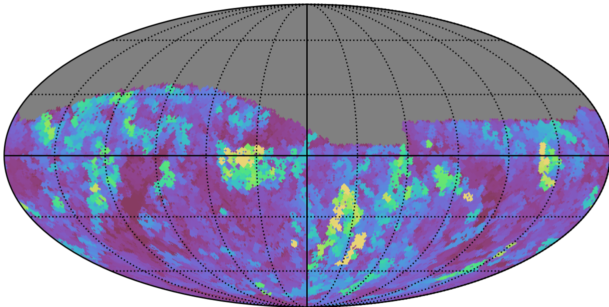
baseline_v3.2_10yrs Yr 1 z band: Max seeingGeom
