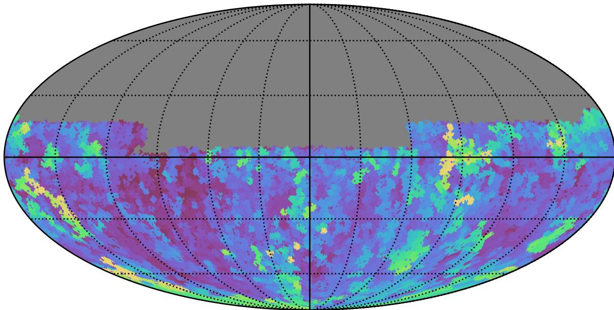
baseline_v3.2_10yrs Yr 1 u band: Max seeingGeom
