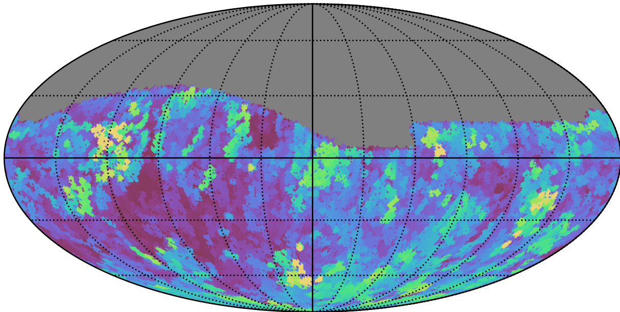
baseline_v3.2_10yrs Yr 1 r band: Max seeingGeom
