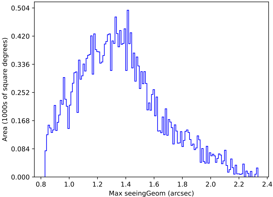
baseline_v3.2_10yrs Yr 1 r band: Max seeingGeom
