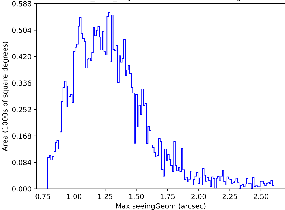
baseline_v3.2_10yrs Yr 1 i band: Max seeingGeom
