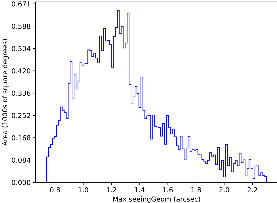
baseline_v3.2_10yrs Yr 1 g band: Max seeingGeom
