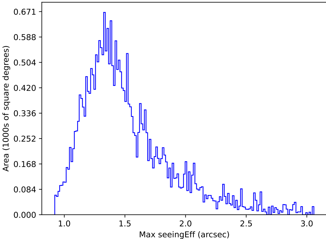
baseline_v3.2_10yrs Yr 1 z band: Max seeingEff
