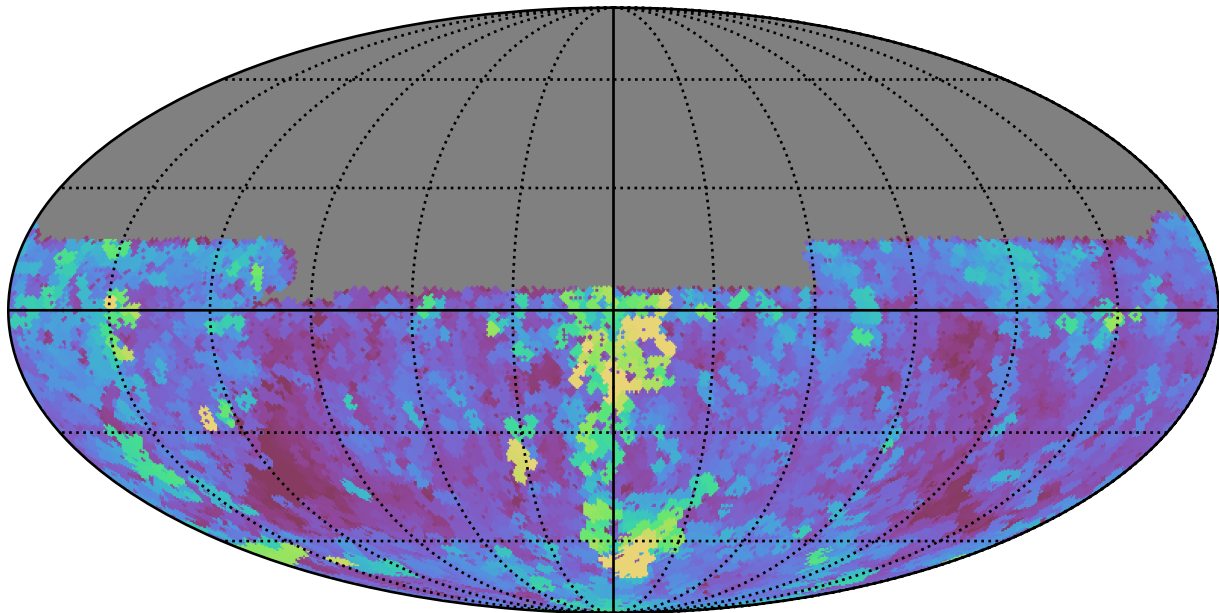
baseline_v3.2_10yrs Yr 1 y band: Max seeingEff
