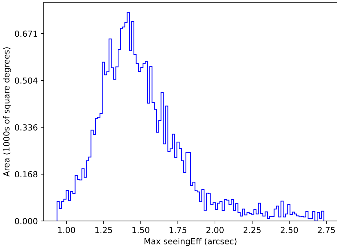
baseline_v3.2_10yrs Yr 1 y band: Max seeingEff
