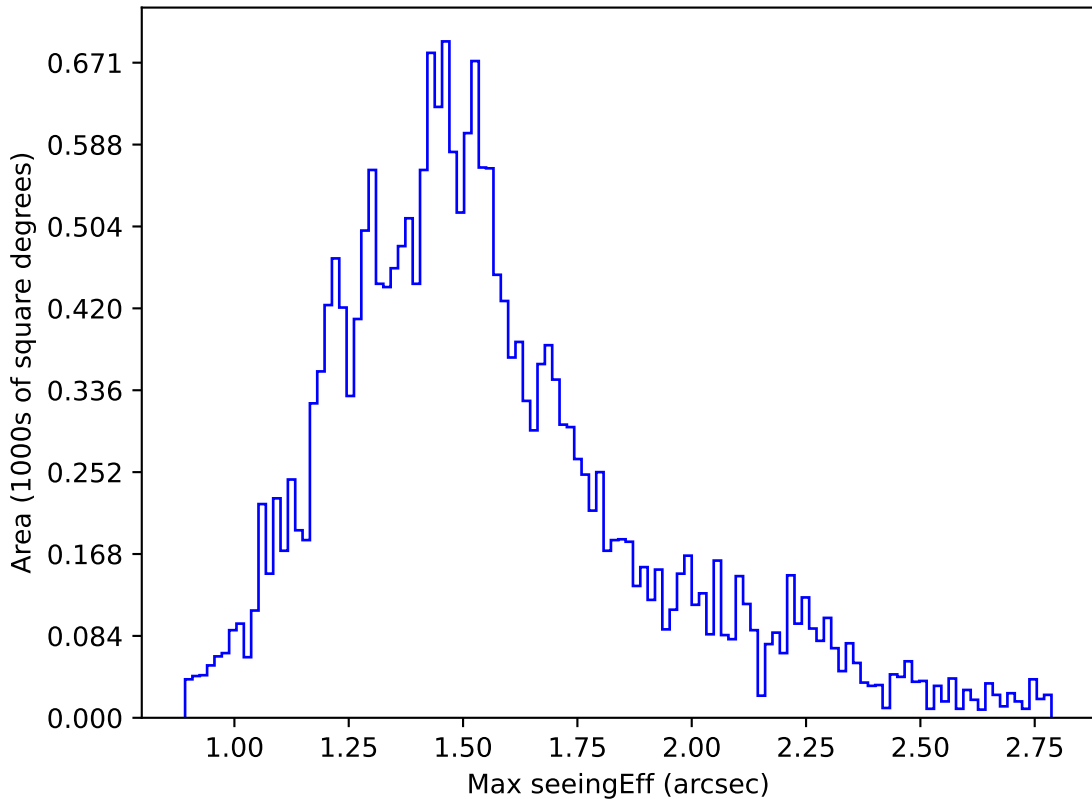
baseline_v3.2_10yrs Yr 1 u band: Max seeingEff
