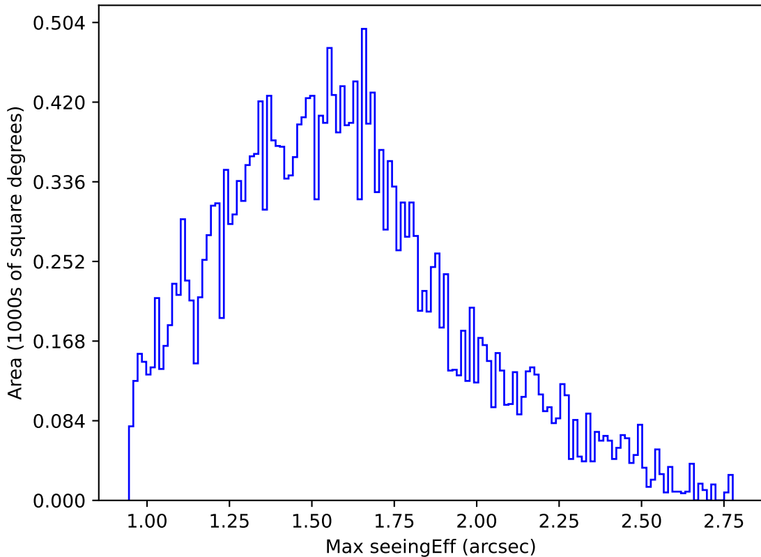
baseline_v3.2_10yrs Yr 1 r band: Max seeingEff
