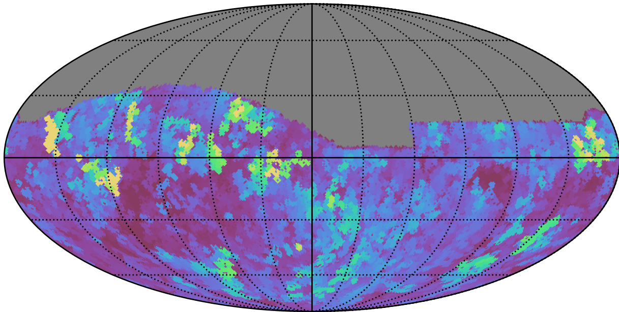
baseline_v3.2_10yrs Yr 1 i band: Max seeingEff
