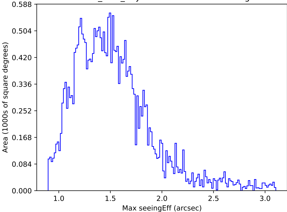
baseline_v3.2_10yrs Yr 1 i band: Max seeingEff
