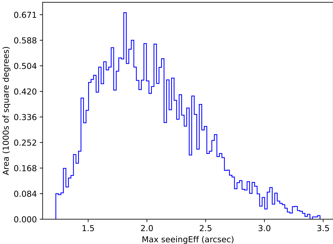
baseline_v3.2_10yrs Yr 1 all bands: Max seeingEff
