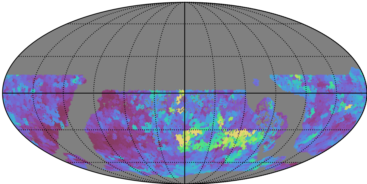
baseline_v3.2_10yrs WFD y band: Max seeingEff
