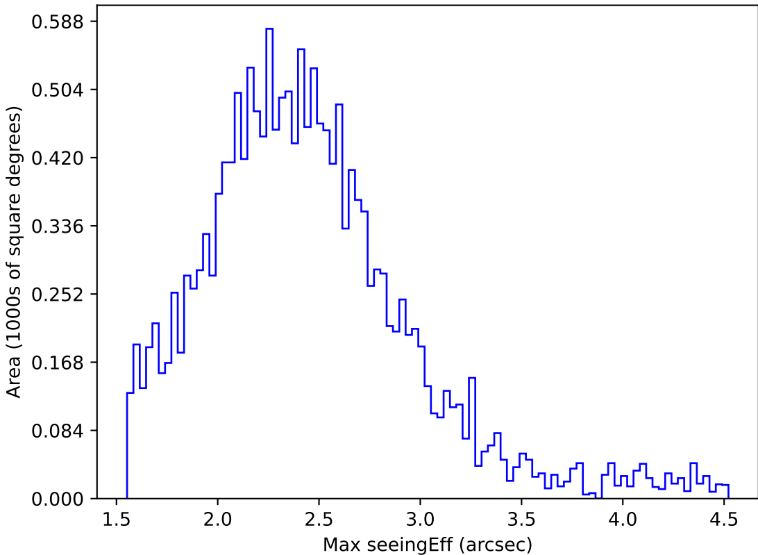
baseline_v3.2_10yrs WFD y band: Max seeingEff
