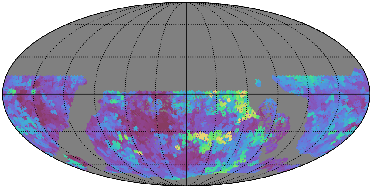
baseline_v3.2_10yrs WFD u band: Max seeingEff
