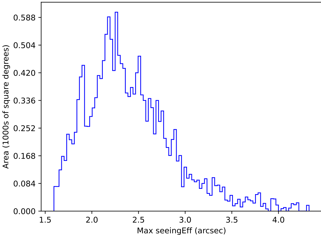
baseline_v3.2_10yrs WFD u band: Max seeingEff
