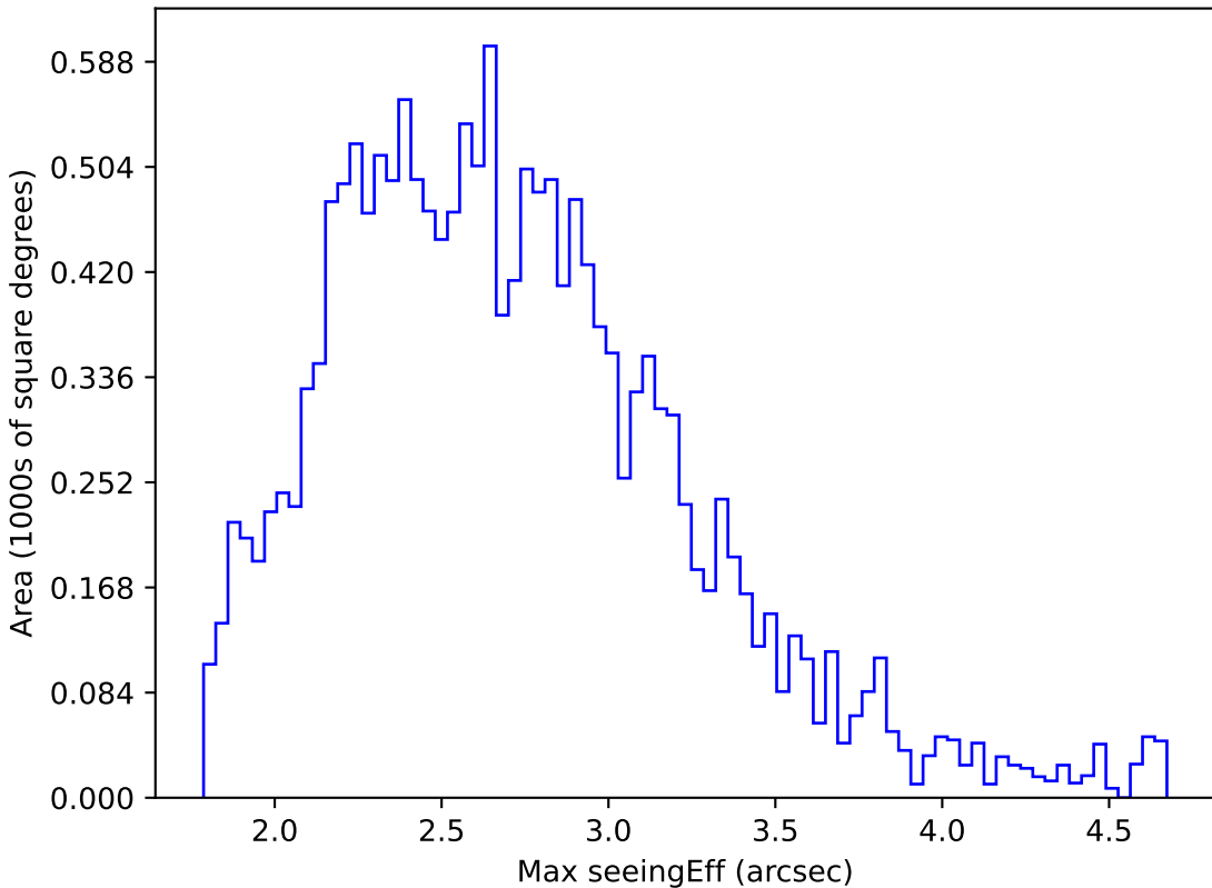
baseline_v3.2_10yrs WFD r band: Max seeingEff
