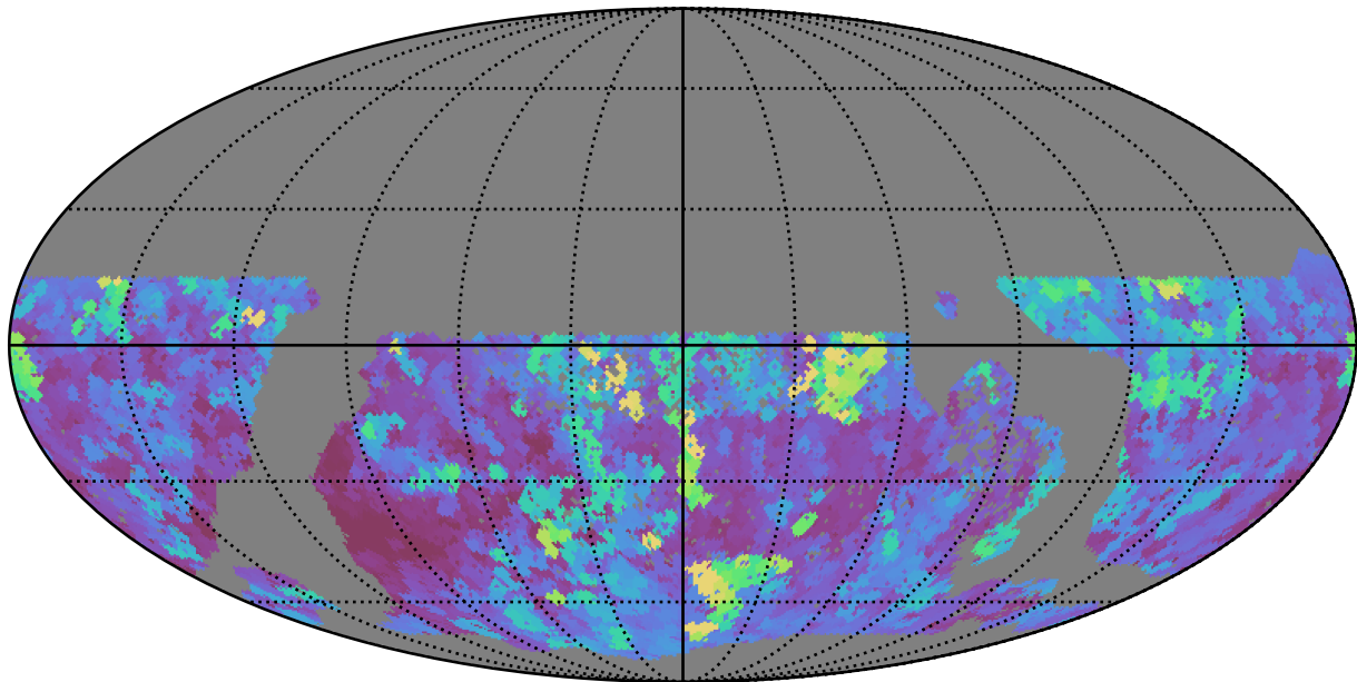
baseline_v3.2_10yrs WFD i band: Max seeingEff
