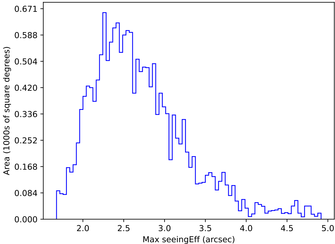
baseline_v3.2_10yrs WFD i band: Max seeingEff
