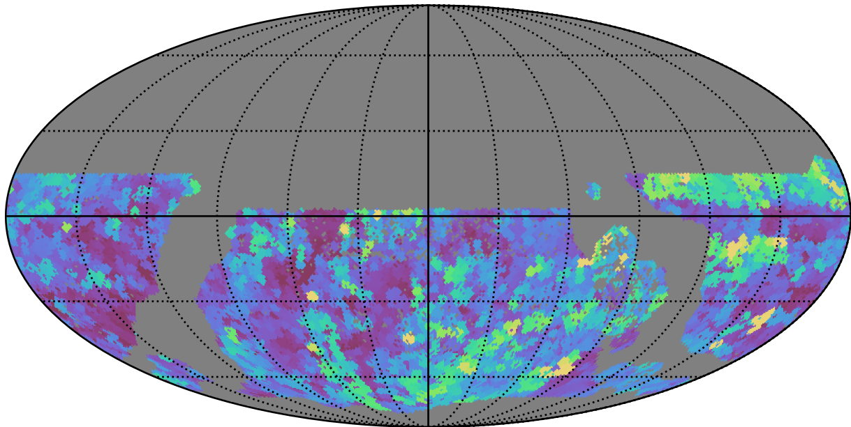
baseline_v3.2_10yrs WFD g band: Max seeingEff
