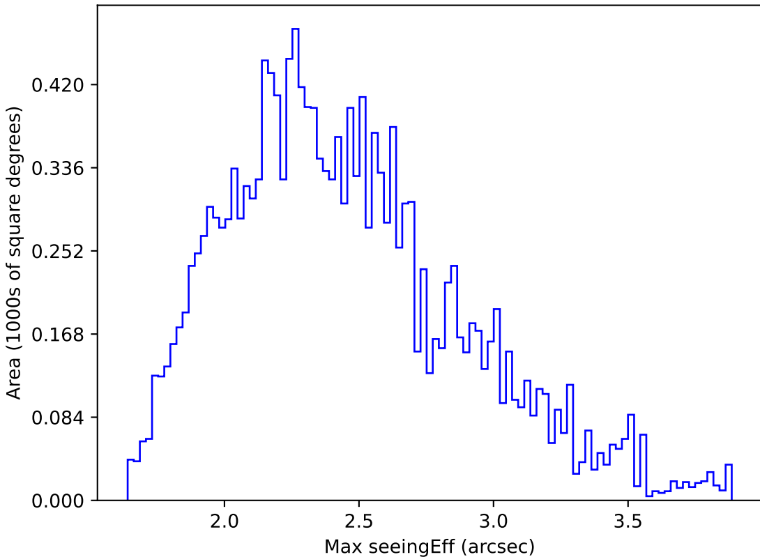
baseline_v3.2_10yrs WFD g band: Max seeingEff
