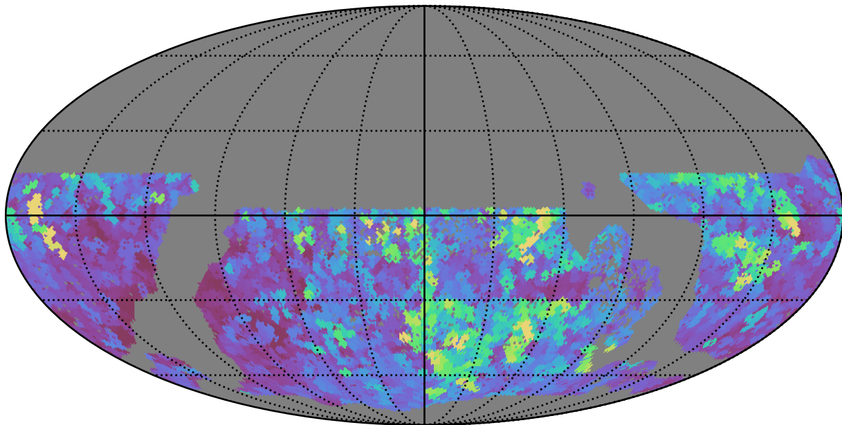
baseline_v3.2_10yrs WFD all bands: Max seeingEff
