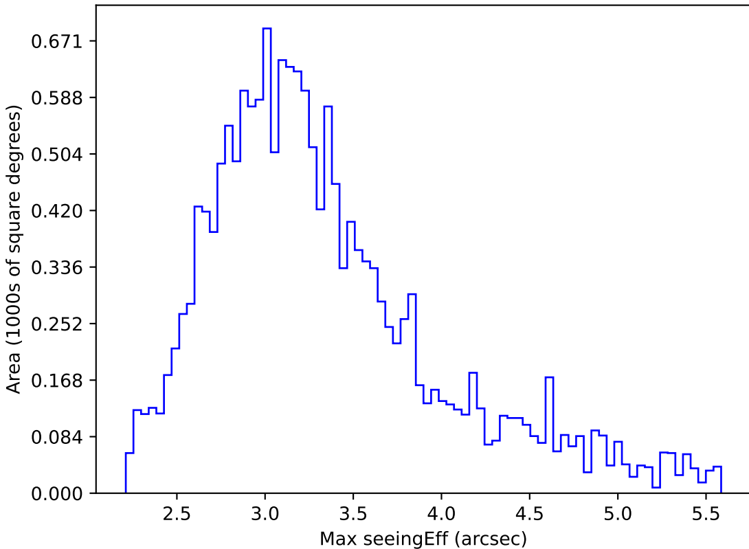
baseline_v3.2_10yrs WFD all bands: Max seeingEff
