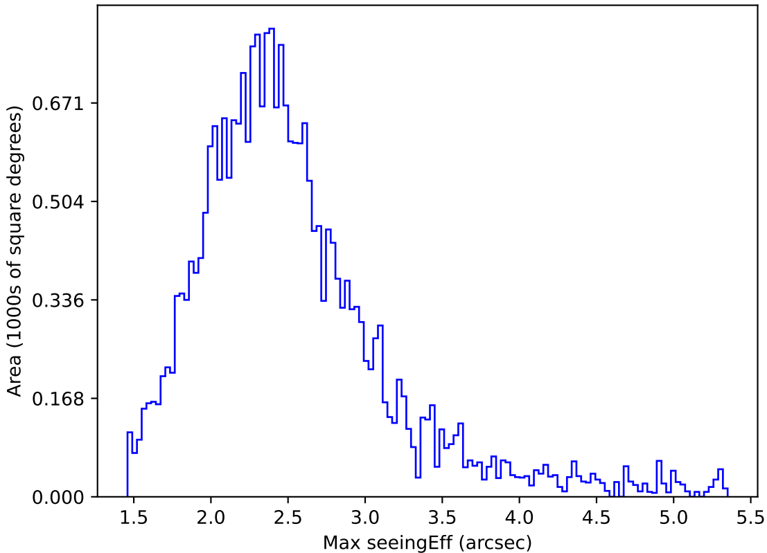
baseline_v3.2_10yrs All sky z band: Max seeingEff
