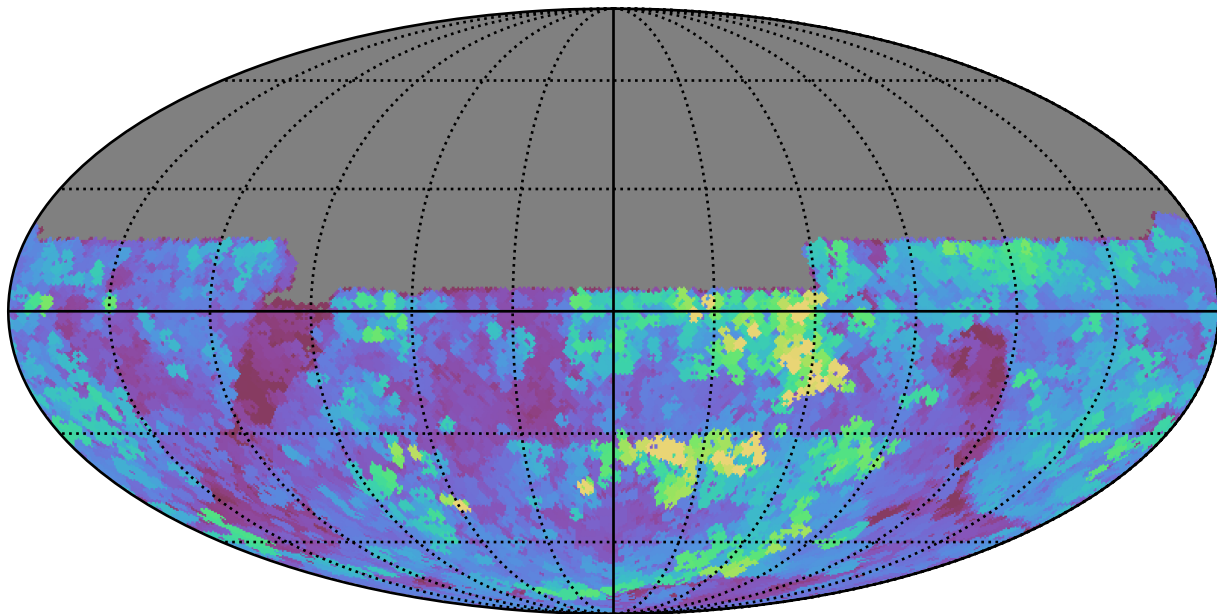
baseline_v3.2_10yrs All sky u band: Max seeingEff
