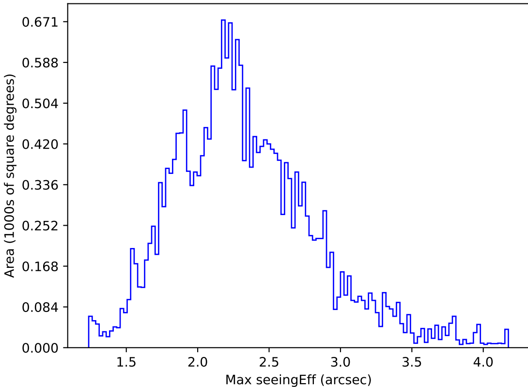
baseline_v3.2_10yrs All sky u band: Max seeingEff
