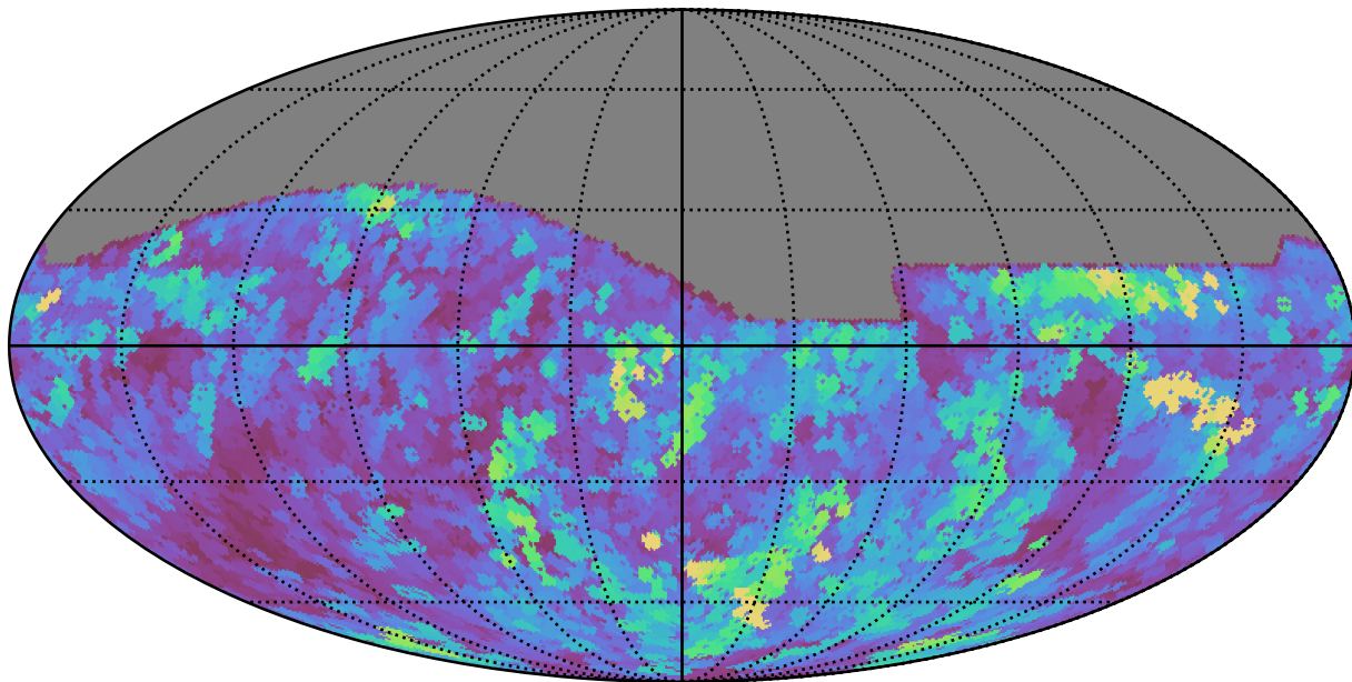
baseline_v3.2_10yrs All sky r band: Max seeingEff
