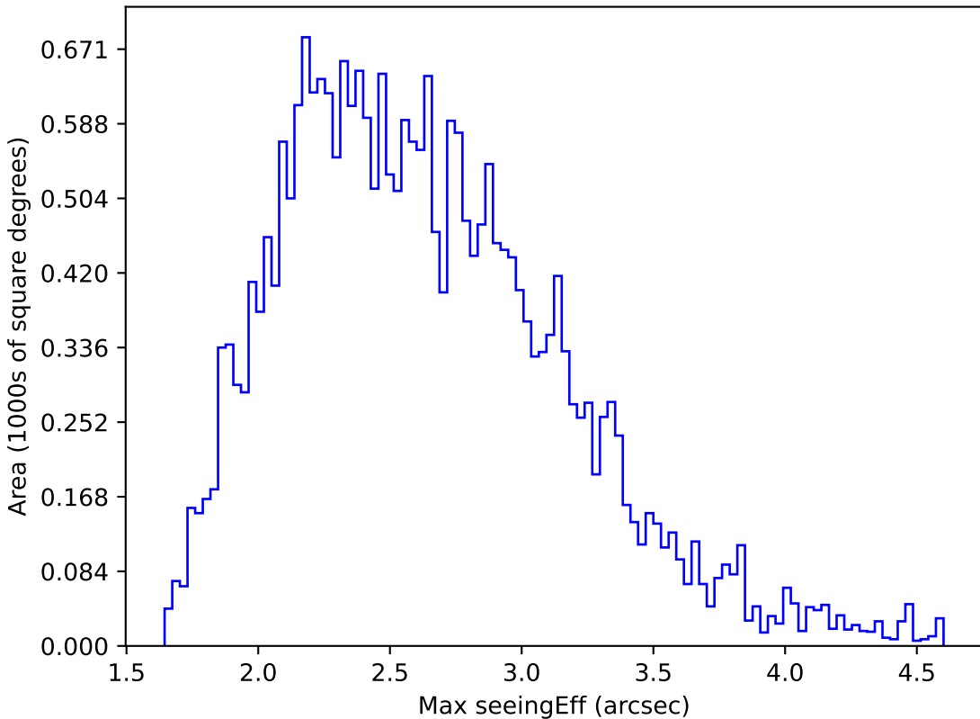
baseline_v3.2_10yrs All sky r band: Max seeingEff
