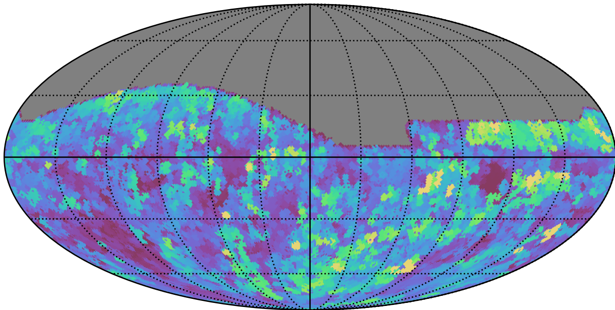
baseline_v3.2_10yrs All sky g band: Max seeingEff
