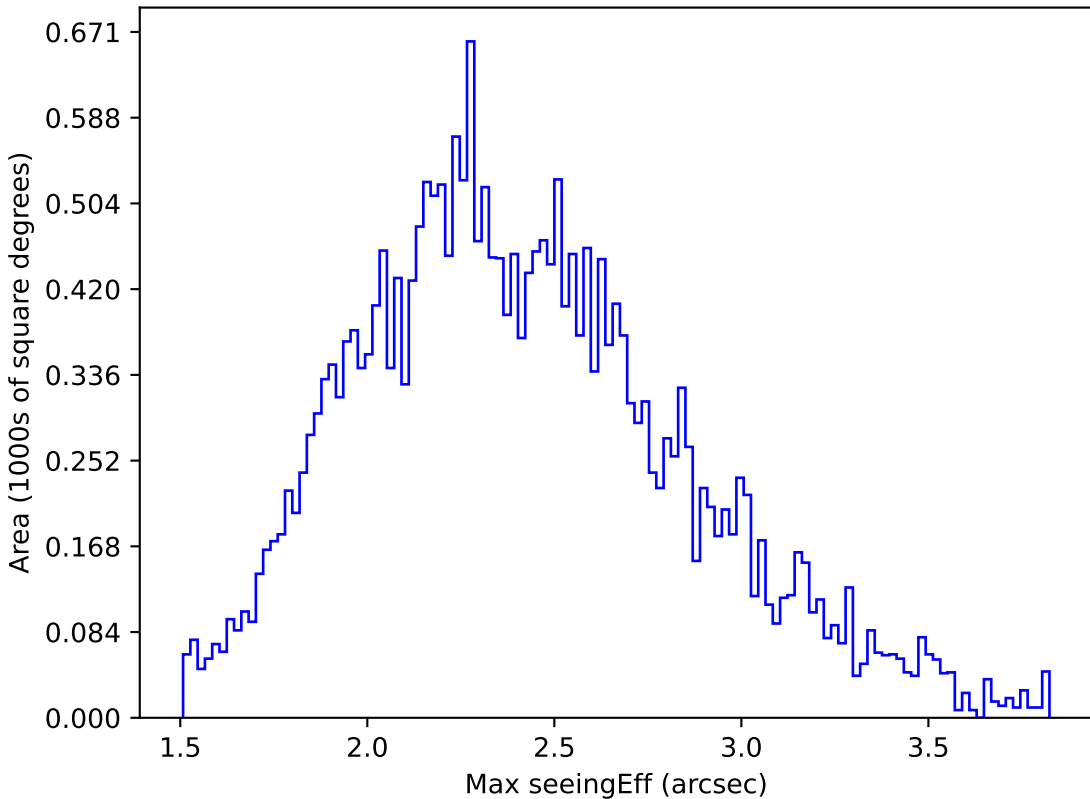
baseline_v3.2_10yrs All sky g band: Max seeingEff
