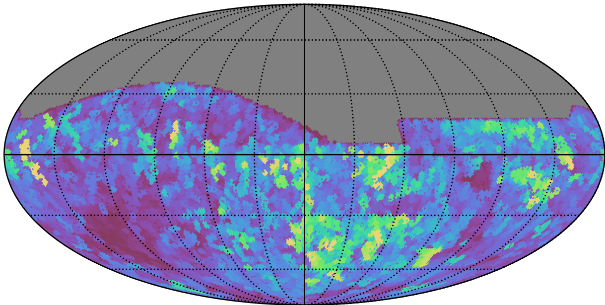
baseline_v3.2_10yrs All sky all bands: Max seeingEff
