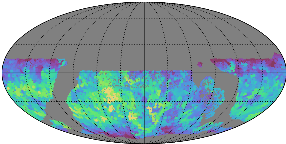
baseline_v3.2_10yrs WFD z band: Max saturation_mag
