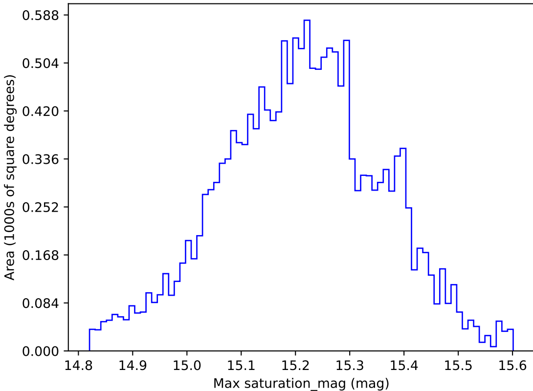
baseline_v3.2_10yrs WFD z band: Max saturation_mag
