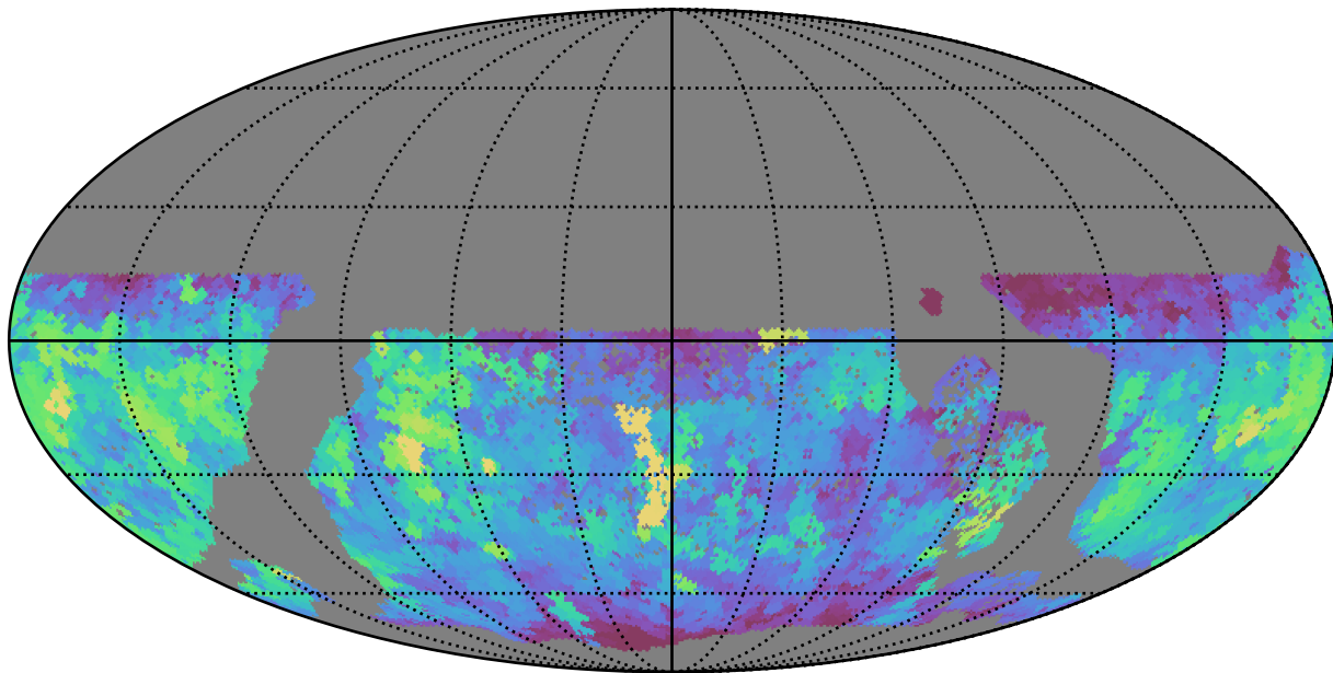
baseline_v3.2_10yrs WFD u band: Max saturation_mag
