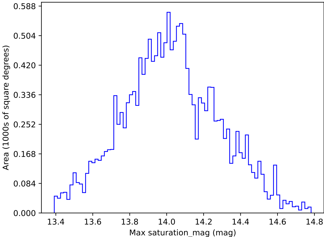
baseline_v3.2_10yrs WFD u band: Max saturation_mag
