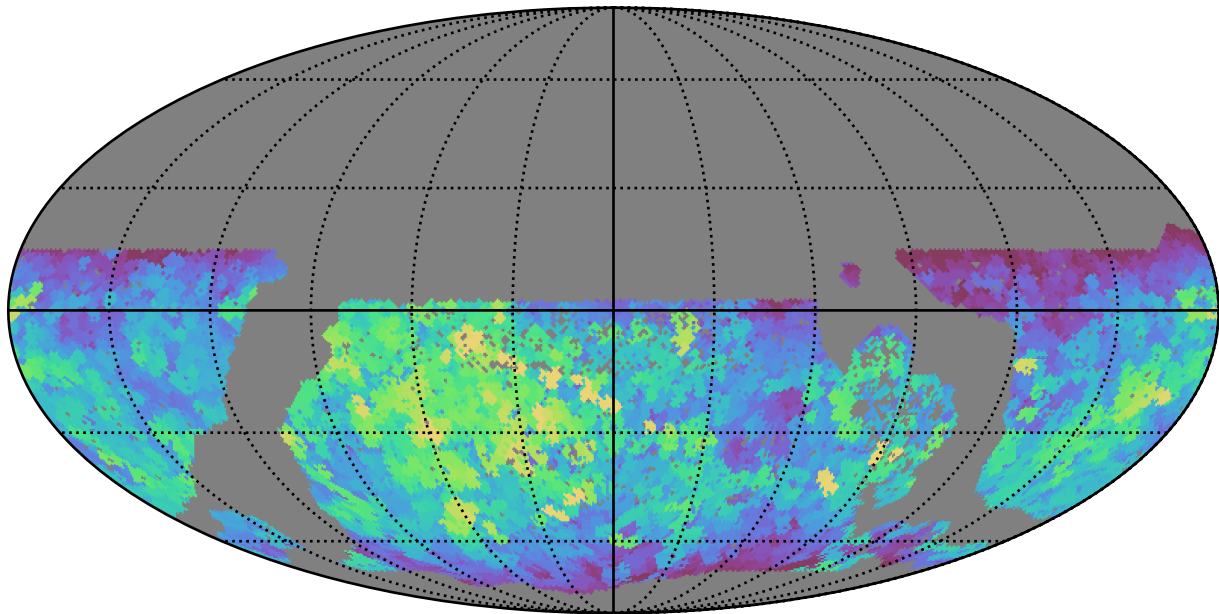
baseline_v3.2_10yrs WFD r band: Max saturation_mag
