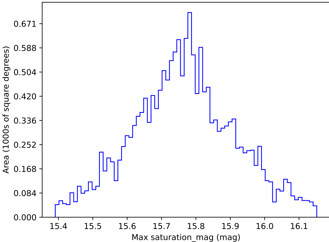
baseline_v3.2_10yrs WFD r band: Max saturation_mag
