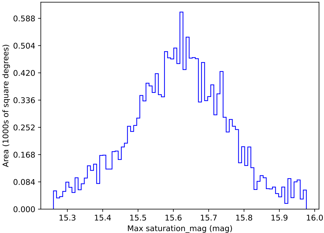
baseline_v3.2_10yrs WFD i band: Max saturation_mag
