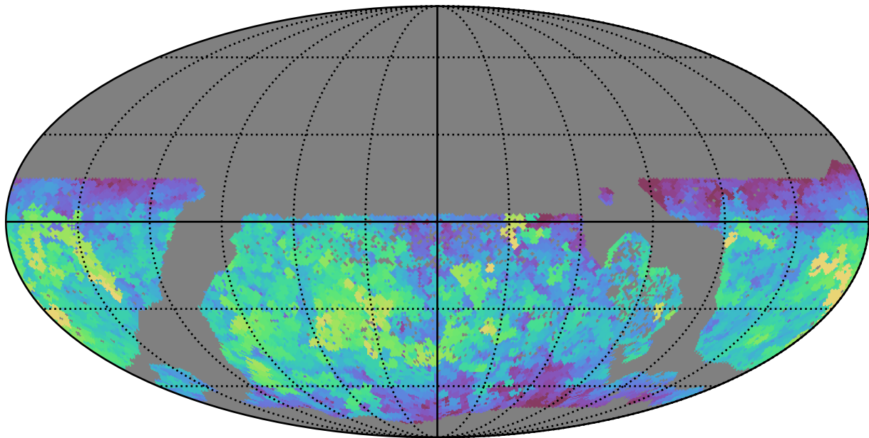
baseline_v3.2_10yrs WFD g band: Max saturation_mag
