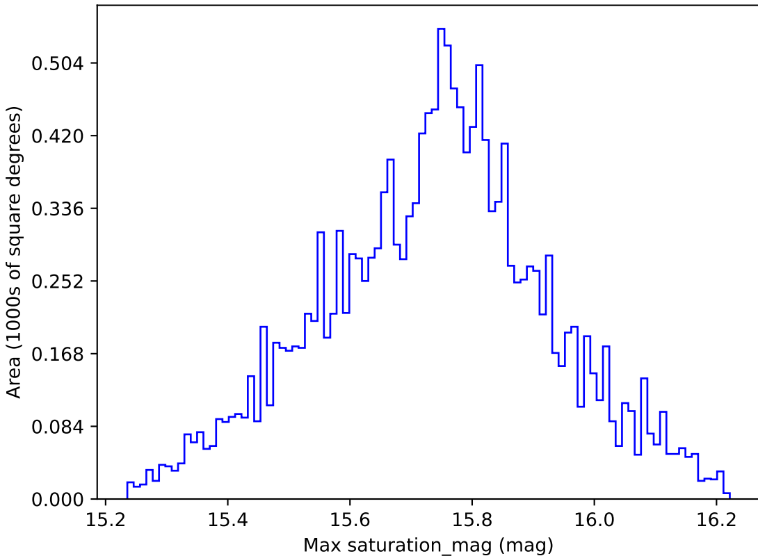
baseline_v3.2_10yrs WFD g band: Max saturation_mag
