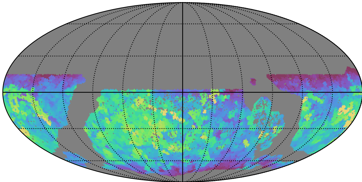
baseline_v3.2_10yrs WFD all bands: Max saturation_mag
