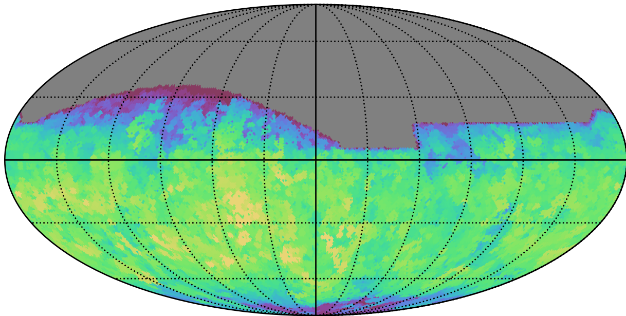
baseline_v3.2_10yrs All sky z band: Max saturation_mag
