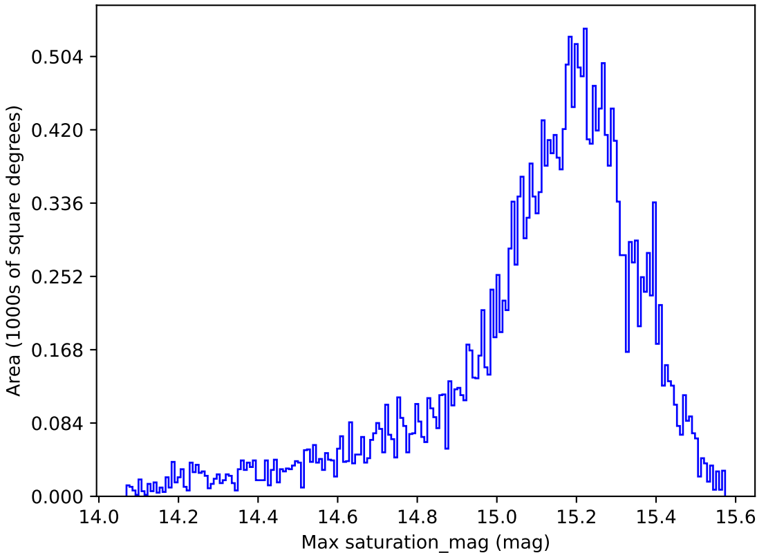
baseline_v3.2_10yrs All sky z band: Max saturation_mag
